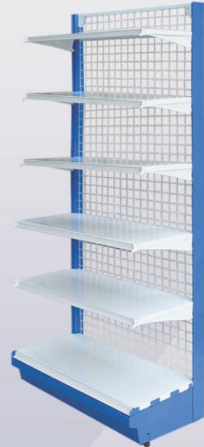
RAK SINGLE WALL / DINDING (6 TINGKAT) Dimension: 90 W × 45 D × 200 H
